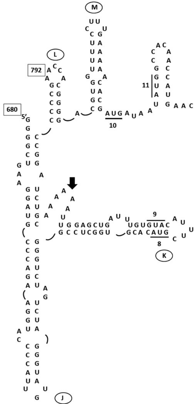
Supplementary Figure S1. Predicted secondary structure of the EMCV IRES (adapted from Duke et al., 1992). The sequences start from position 680. Circled capital letter J, K, L and M indicate defined region in the IRES. Arrow indicates the A bulge in the J-K domain. AUG8, AUG9, AUG10 and AUG11 are underlined.
