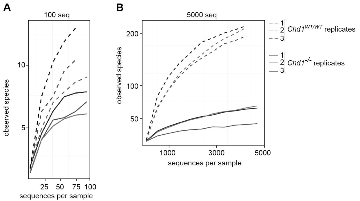
S3 Fig. Rarefaction curves for capped sequence data sets. (A) Capping the sequence number to 100 per sample indicates insufficient discriminatory power. (B) Capping sequence number to 5000 per sample suggests representative sampling and improves discrimination of Chd1 -/- and Chd1 WT/WT associated microbiota.
