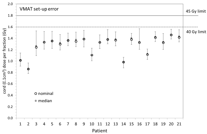
Supplementary Figure Cord dose ( 0.1\text{cm}^3 ) robustness for each patient for the nominal plans (circles), with perturbed plans median dose (squares) and maximum /minimum values (error bars). Top : VMAT set-up error; middle : SFO set-up error and bottom : SFO range error.
