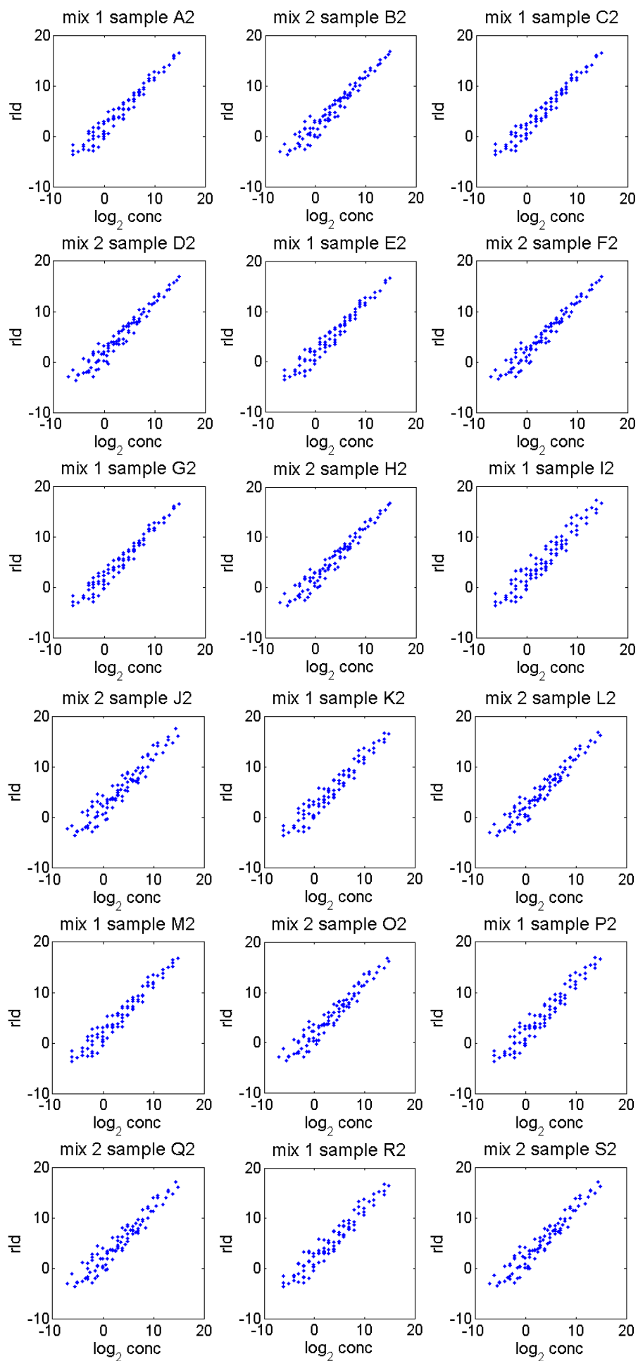
Fig. S1 Relationship between ERCC rld normalized counts and their nominal concentration
