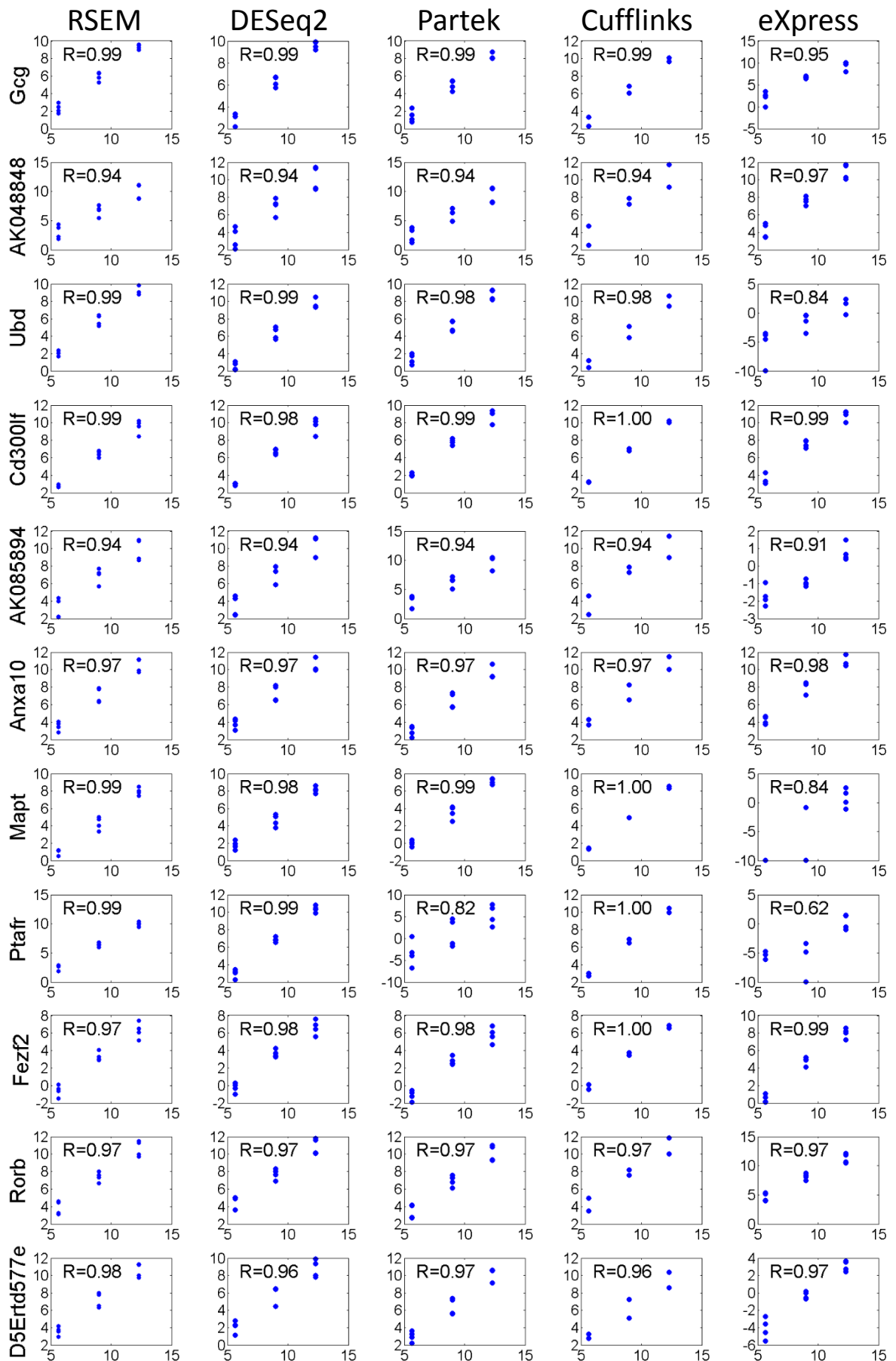
Fig. S3 Scatter plots of mouse single locus spikes: expected vs. observed concentrations
