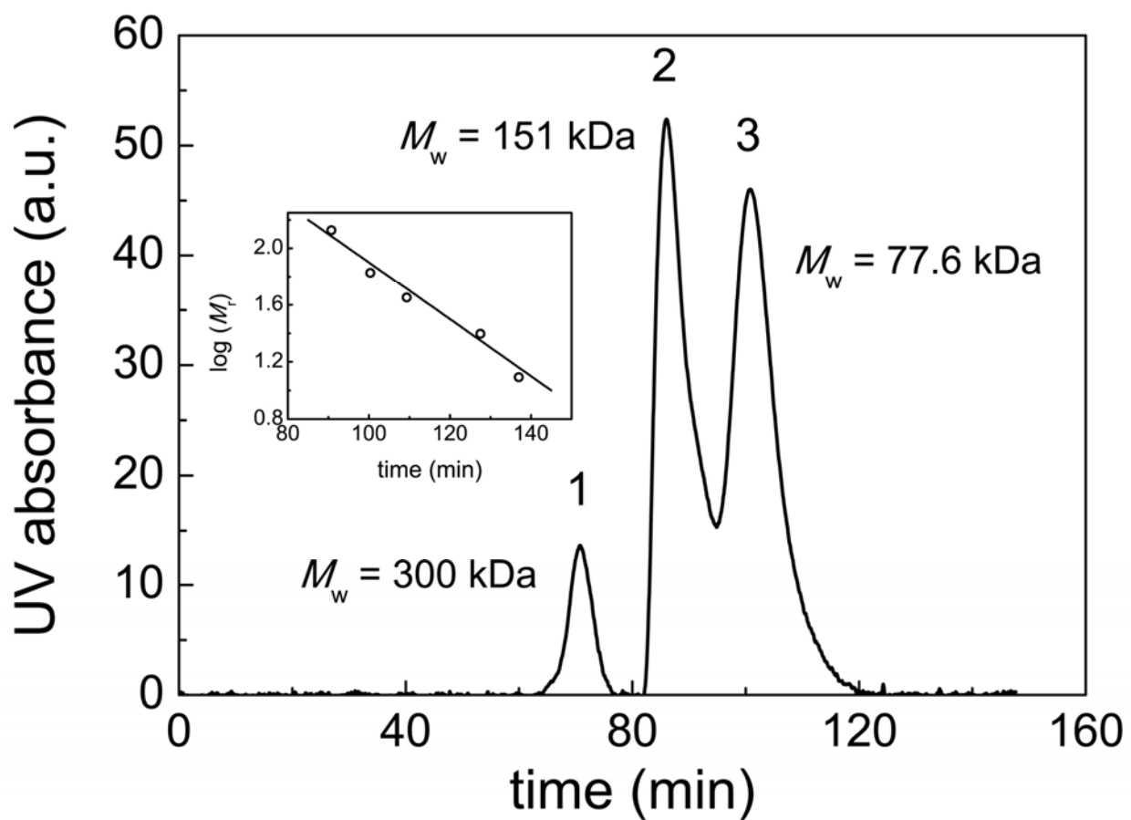
S1 Fig. SEC elution profile (Sephacryl S100 HR, flow rate of 2.5 ml/min, 20 °C) for non-aggregated BSA obtained after heating for 12 h at 60 °C.
