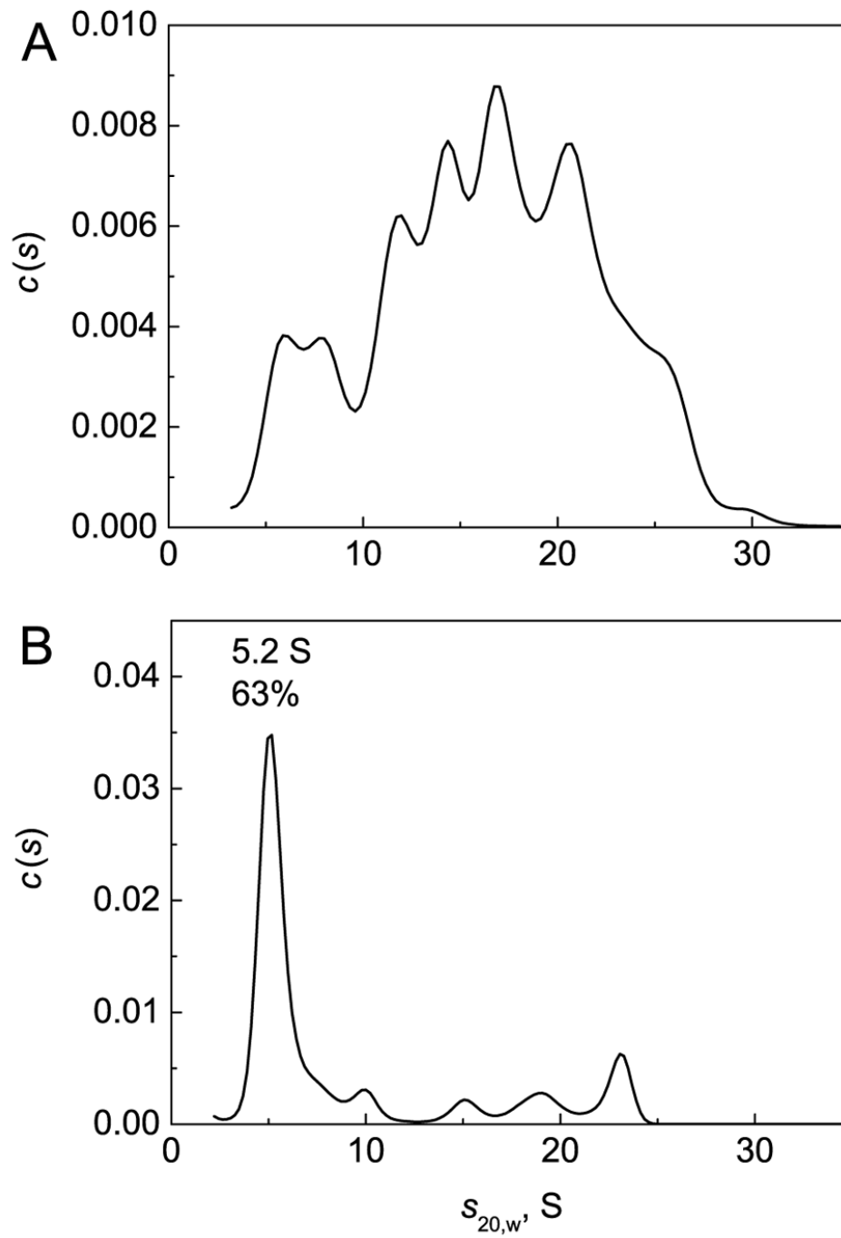
S2 Fig. Analytical ultracentrifugation of SEC-obtained fractions of BSA preheated for 12 h at 60 °C.
