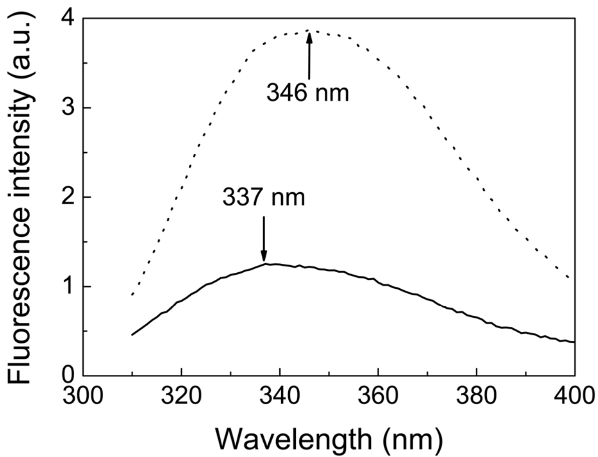
S4 Fig. Tryptophan fluorescence spectra for intact BSA (dotted line) and non-aggregated unfolded BSA (solid curve).
