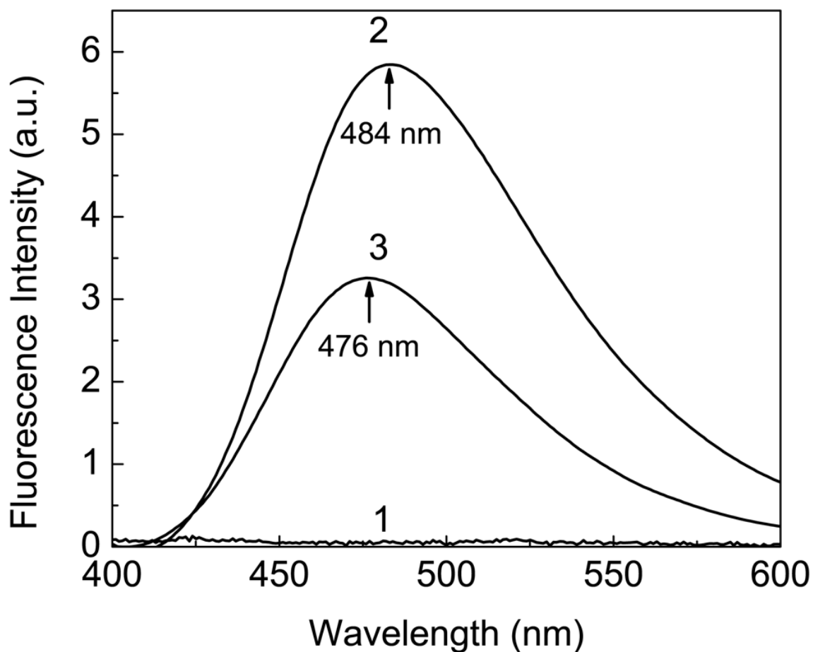
S5 Fig. Fluorescence spectra of free ANS (10 \mu M; curve 1), ANS (10 \mu M) in the presence of intact BSA (0.1 mg/ml; curve 2) and ANS (10 \mu M) in the presence of non-aggregated unfolded BSA (0.1 mg/ml; curve 3).
