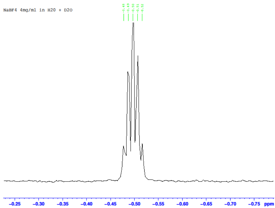
Expanded view of 11 B NMR spectrum of NaBF 4 (4 mg/mL) in neutral H 2 O/D 2 O
