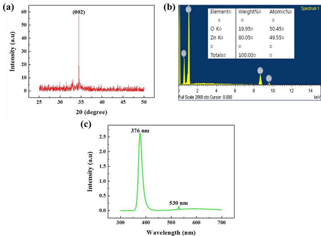
Figure S2. (a) XRD, (b) EDS, and (c) PL spectra of ZNRs grown with the microwave-assisted solution-replacement method.
