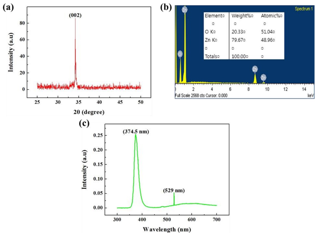
Figure S3. (a) XRD, (b) EDS, and (c) PL spectra of ZNRs grown with the microwave-assisted preheating method.
