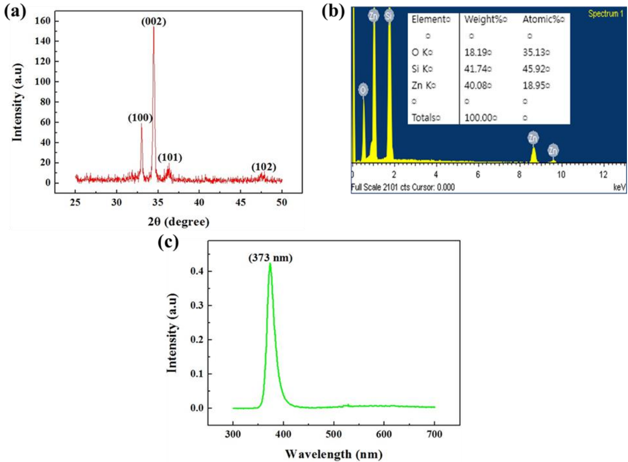
Figure S1. (a) XRD, (b) EDS, and (c) PL spectra of ZNRs grown with the microwave-assisted direct growth method.
