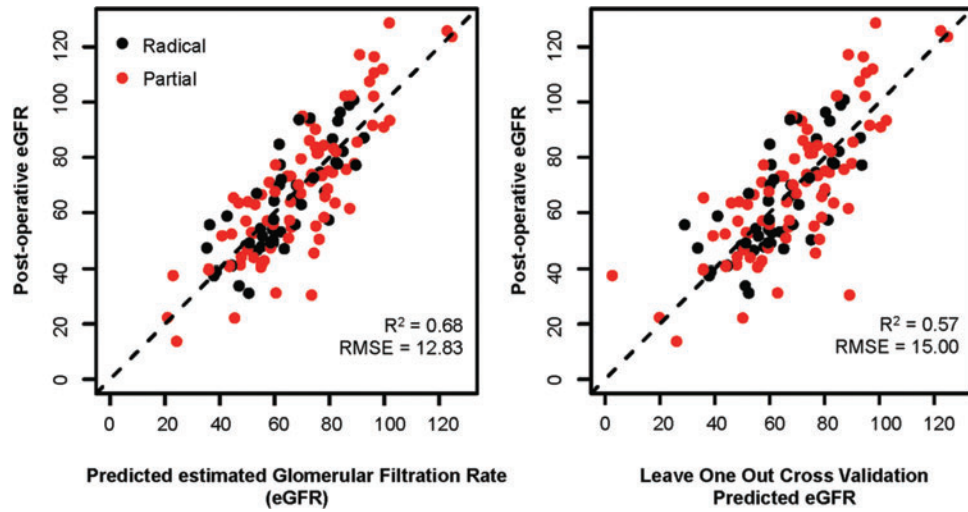
SUPPLEMENTARY FIG. S2. ( Left ) Model predictions of eGFR at 6 months after surgery. Scatter plot of actual compared with predicted eGFR in our cohort with a regression line to determine correlation. ( Right ) Using the leave-one-out cross-validation. Scatter plot of actual compared with predicted model using leave-one-out cross validation in our cohort with a regression line to determine correlation and assume no overfitting. RMSE=root mean square error.
