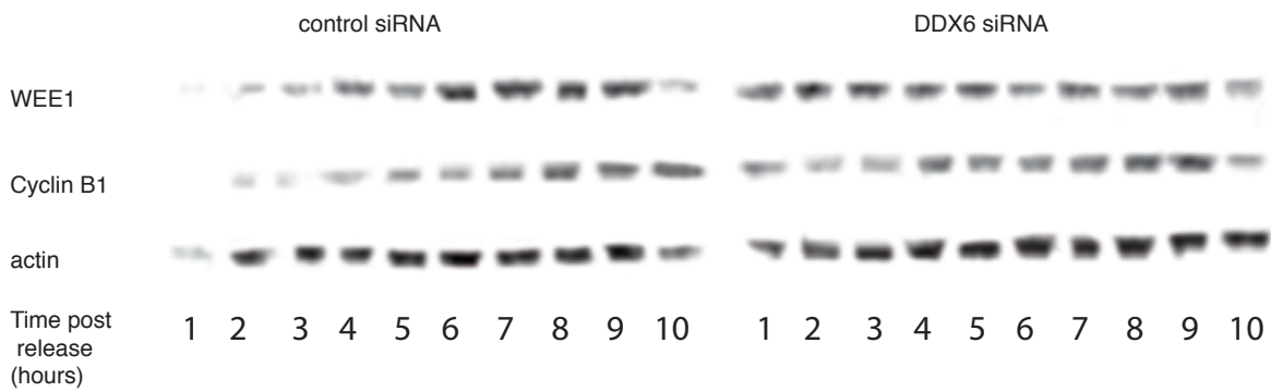
Figure S7. Differential expression of WEE1 along the cell cycle is dependent on DDX6. HeLa cells were transfected with control SiRNA and DDX6 SiRNA, Cells were synchronized by double thymidin block. Western blot analyses of WEE1 and cyclin B1 expression were performed at each hour after release from the double thymidine block!
