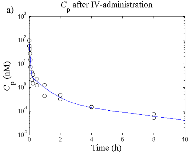
Figure S1 a) Plasma concentration ( C_p ) after intravenous (IV) administration of fluticasone propionate (FP) to rats (90 nmol/kg, n = 2 ), and b) concentration of receptor-drug complex in the spleen ( RD_{spleen} ) after IV-administration of FP (90 nmol/kg, n = 3 /time point). Observed data are indicated by circles and the model fit by a solid line.
