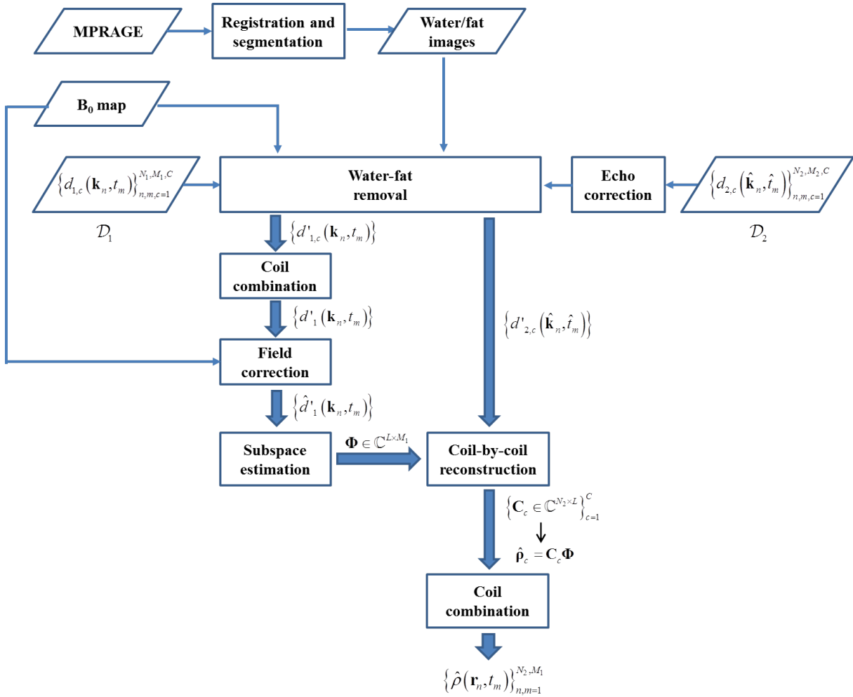
Figure S1: Data processing pipeline for ^1\text{H} -MRSI of the brain using SPICE. The lower case letter c denotes the coil index. d'_{1,c}(\cdot) and d'_{2,c}(\cdot) denote the water-fat removed D_1 and D_2 for all the coils. The variables without the coil index denote the data after coil combination.
