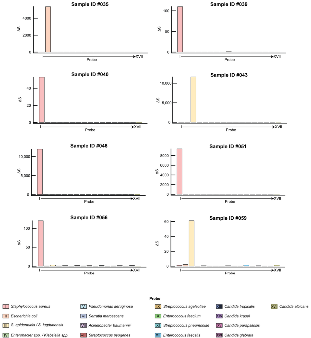
Figure S3 - Performance of PID assay with concordant culture positive clinical specimens. Sample numbers refer to patient specimens listed in Tables 1 and S3. Sample ID #035, #039, #040, #043, #046, #051, #056, #059 were deemed positive for E. coli , S. aureus , S. aureus , CoNS, S. aureus , S. aureus , S. aureus , and CoNS, respectively.
