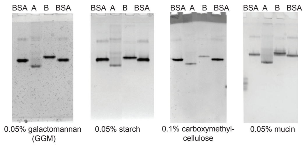
Figure S1: Affinity PAGE with glycans that are not recognized by SGBP-A and SGBP-B. Affinity electrophoresis (10% acrylamide) of SGBP-A and SGBP-B with BSA as a control protein. The percent polysaccharide incorporated into each native gel is displayed.
