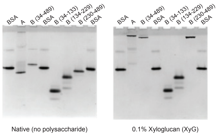
Figure S5: Affinity PAGE with glycans that are not recognized by SGBP-A and SGBP-B. Affinity electrophoresis (10% acrylamide, native and 0.1% XyG) of SGBP-A and SGBP-B full length (34-489) and truncated proteins expressing domain A (34-133), domain B (134-229), or domains CD (230-489). BSA was included as a control protein.
