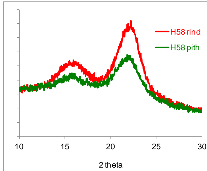
Fig. S2. Illustrative X-ray diffraction spectra of the rind (red) and pith (green) regions of the sugarcane hybrid 58.
