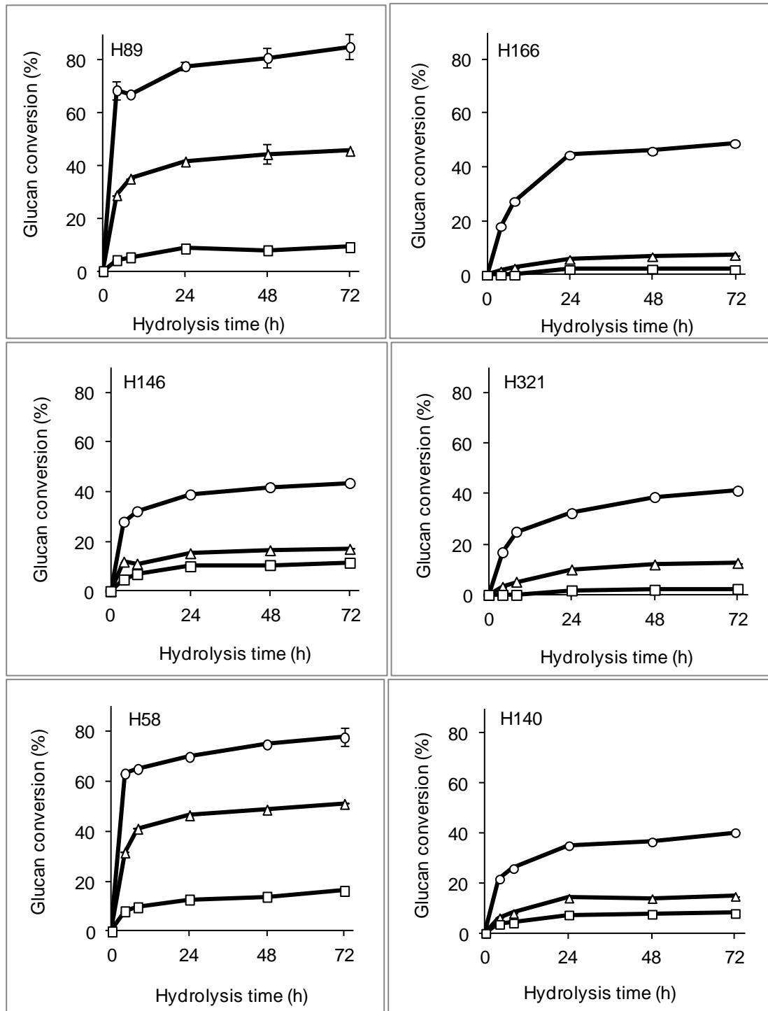
Fig. S3. Time-dependence of the enzymatic conversion of glucan to glucose in internode fractions from six different sugarcane hybrids. Error bars represent the standard deviations for triplicate hydrolysis experiments. Symbols: (circles) pith, (triangles) pith-rind interface, (squares) rind.
