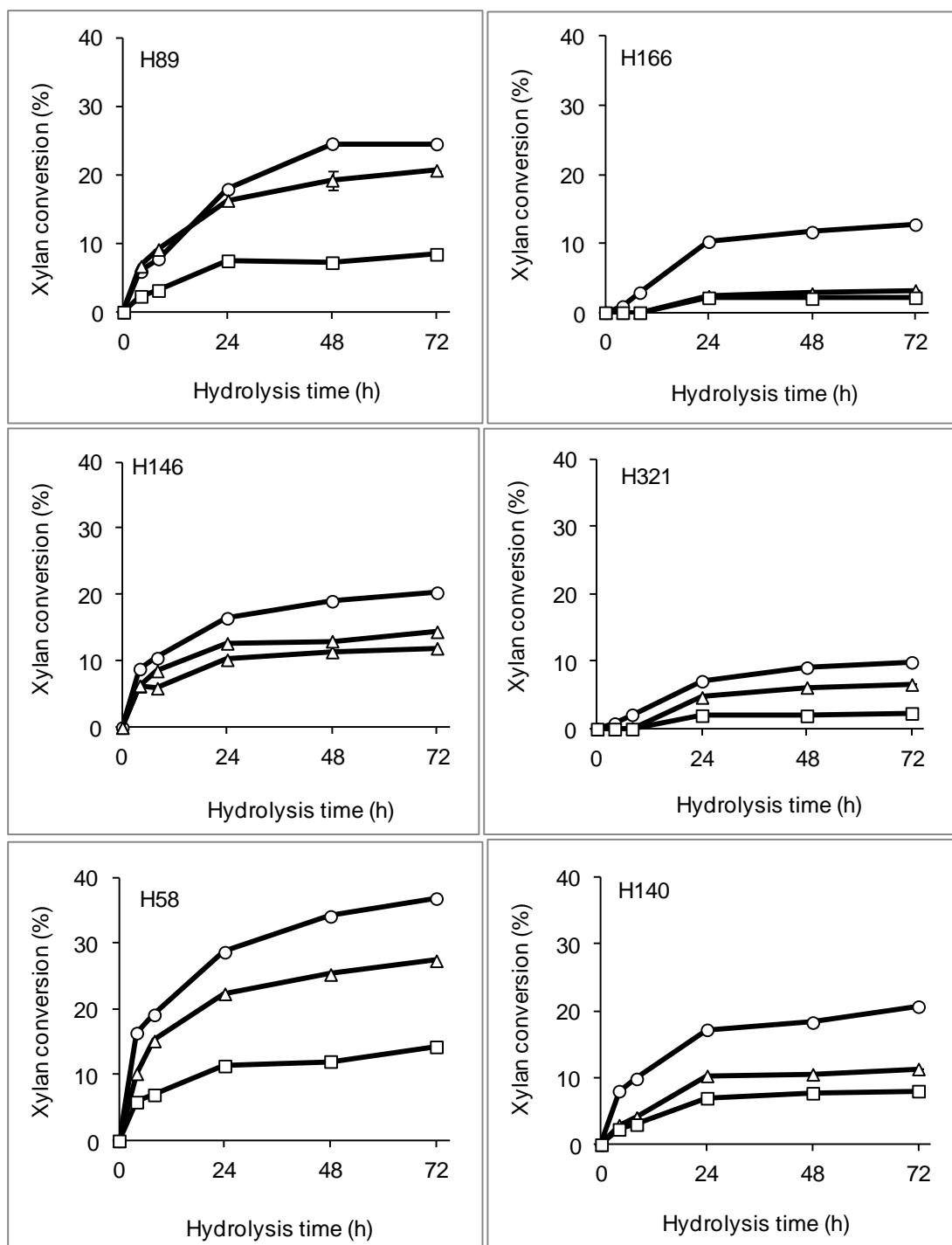
Fig. S4. Time-dependence of the enzymatic conversion of xylan to xylose in internode fractions from six different sugarcane hybrids. Error bars represent the standard deviations for triplicate hydrolysis experiments. Symbols: (circles) pith, (triangles) pith-rind interface, (squares) rind.
