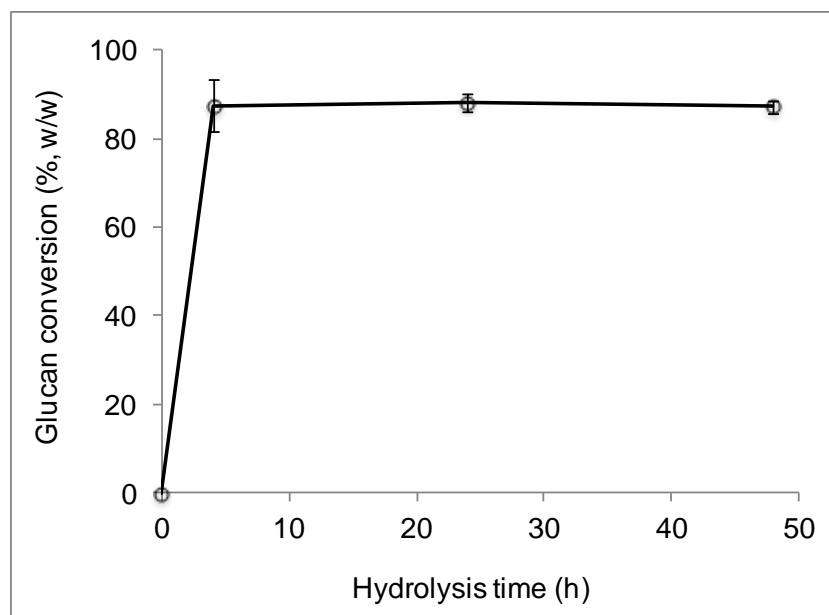
Fig. S5. Time dependence of the enzymatic conversion of barley MLG to glucose monomers with commercial enzymes. Error bars represent the standard deviations for triplicate hydrolysis experiments.
