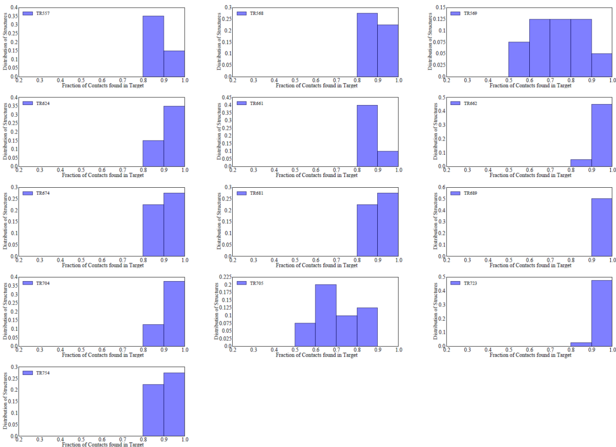
Figure S1 shows the fraction of contacts retained from the target structure for each snapshot obtained during unfolding by FRODA. We find that there are generally very few structures found in any given unfolding trajectory that retain less than 50% of the original target structure's contacts.
