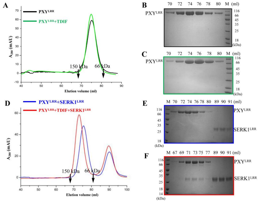
Supplementary information, Figure S6 TDIF induces PXY LRR and SERK1 LRR interaction in vitro . (A-C) TDIF induces no PXY LRR homodimerization. Right: Coomassie blue staining of the peak fractions shown on the left following SDS-PAGE. (D-F) TDIF induces PXY LRR and SERK1 LRR heterodimerization. Right: Coomassie blue staining of the peak fractions shown on the left following SDS-PAGE. “M”: molecular weight ladder (kDa).
