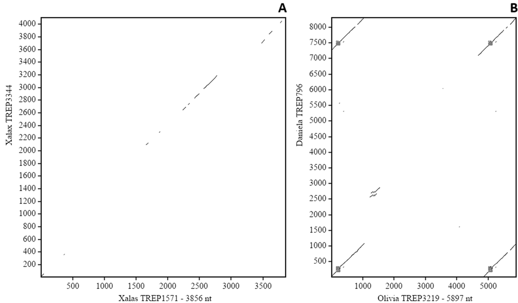
Additional file 2. Dot-plot alignment of TE sequences most highly enriched in the TE/tandem array junctions.
