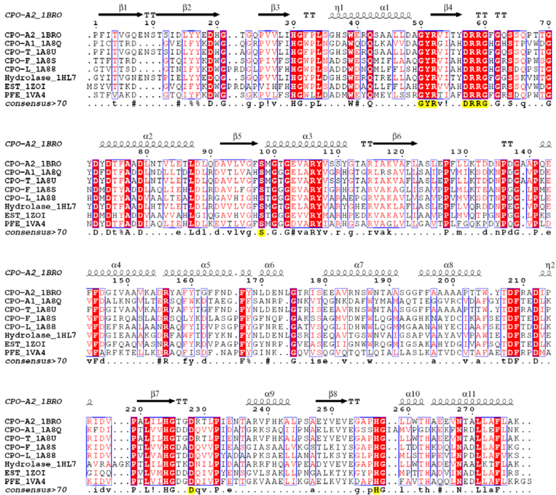
S2 Fig. Multiple sequence alignment of the cofactor-free HPO and the \alpha/\beta hydrolases. The conserved residues include the GYR and DRRG motifs, the catalytic triad (S98-D228-H257), and the residues (HG, D-G-G-S and G-S-G-G) for structure arrangement and stabilization.
