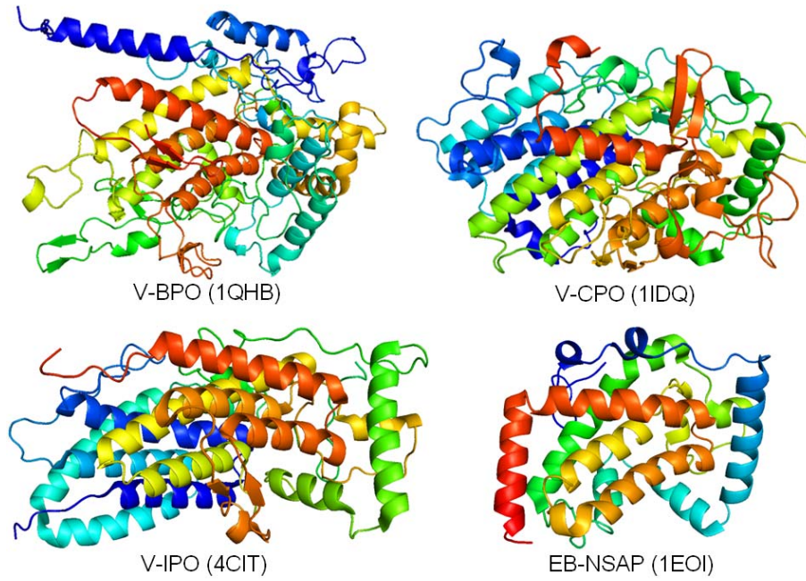
S6 Fig. Structure comparison of the V-HPO and the acid phosphatase.
