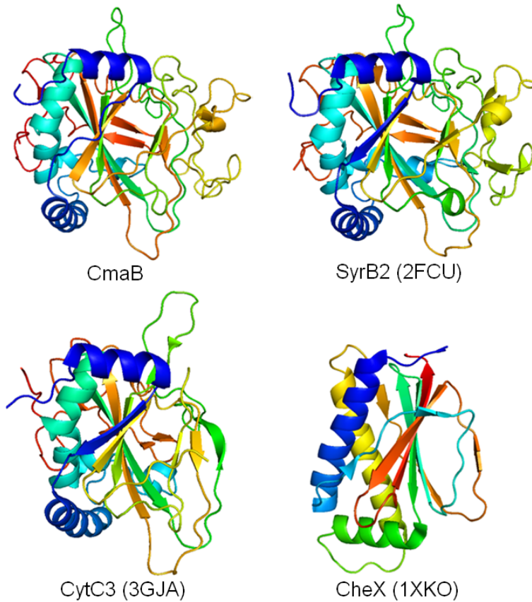
S10 Fig. Structure comparison of the NI-HG and the chemotaxis phosphatase. The structure of CmaB (AAO58149) from Pseudomonas syringae was predicted based on the crystal structure of SyrB2 (2FCU), using the SWISS-MODEL homology-modeling server.
