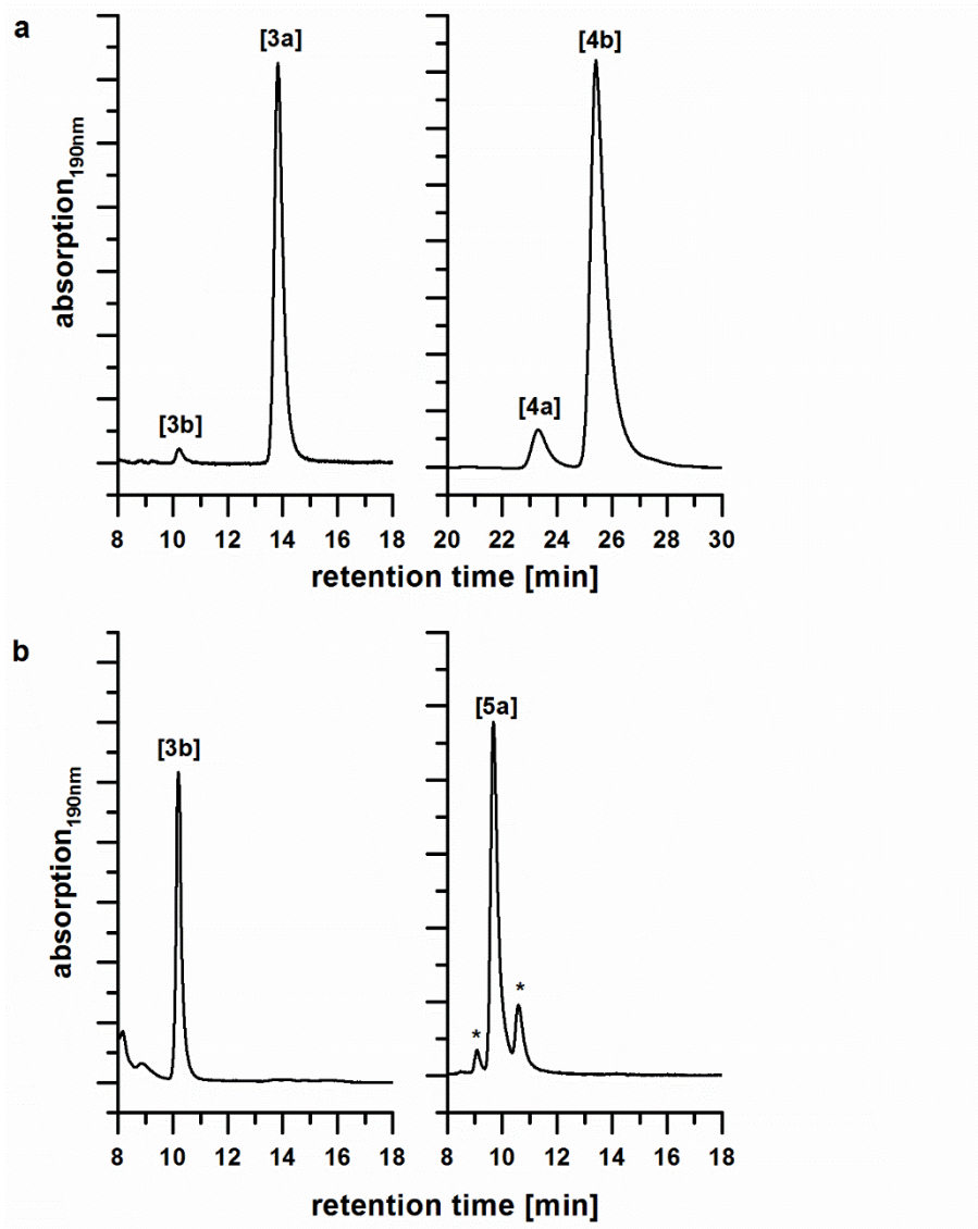
Additional file 5: HPLC chromatograms of enantiomeric separations of reaction products. a Application of AtPrR2; b application of FiPLR. [3a] = (+)-pinoresinol 3a , [3b] = (-)-pinoresinol 3b , [4a] = (+)-lariciresinol 4a , [4b] = (-)-lariciresinol 4b , [5a] = (-)-secoisolariciresinol 5a .
