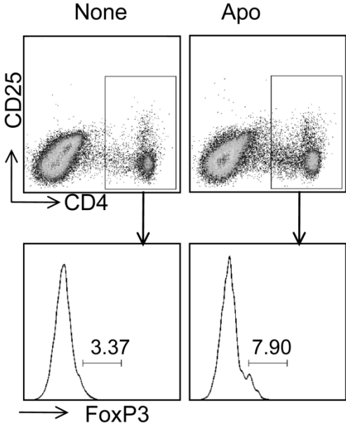
Percentage of FoxP3 + cell in CD4 gated cells
