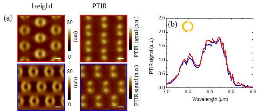
Figure S1-Sn. (a) Pairs of height (left column) and PTIR (right column) images obtained at 1142 \text{ cm}^{-1} for vertically shifted and horizontally shifted centered rectangular A-SRR arrays. The PTIR images are displayed with common intensity scale and all scale bars are 1 \mu\text{m} . (b)-(c) Normalized PTIR spectra obtained at the hot spot locations of vertically (red) and horizontally shifted (blue) centered rectangular arrays for A-SRR (b) See the detailed normalization procedure in the experimental.
