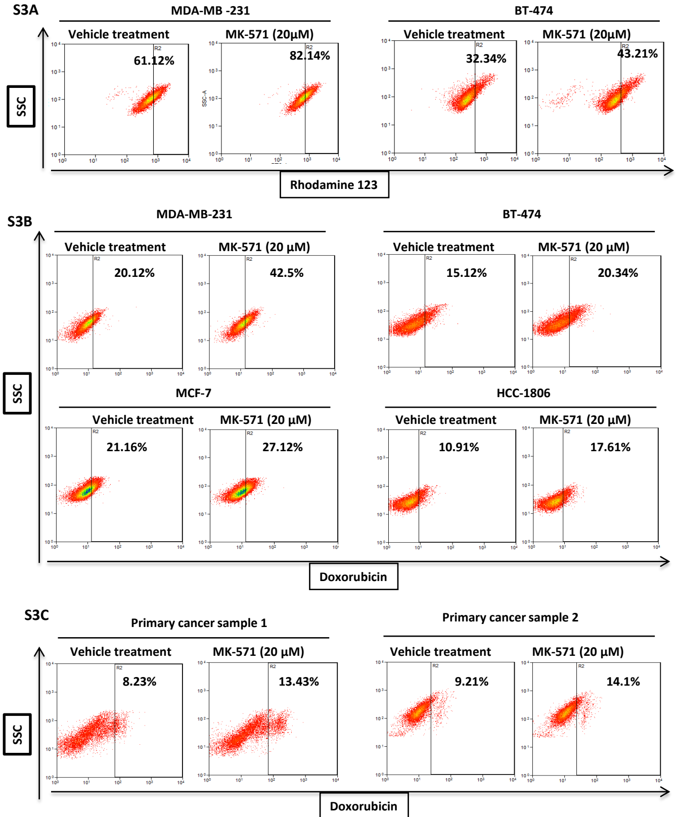
S3 Fig. Effect of MK-571 on Rhodamine and Doxorubicin retention in breast cancer cells: FACS plots represents rhodamine-123 retention in MK-571 treated breast-cancer cells (S3A), doxorubicin retention in MK-571 treated breast cancer cells (S3B) and in primary breast cancer cells (S3C). n=3.
