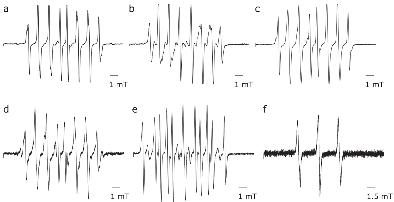
Supplemental. Fig. 1. Typical representative ESR spectra of (a) \cdot\text{OH} , (b) \text{O}_2^{\cdot-} , (c) \text{RO}\cdot , (d) \text{ROO}\cdot , (e) \text{R}\cdot and (f) ^1\text{O}_2 observed in the study.
