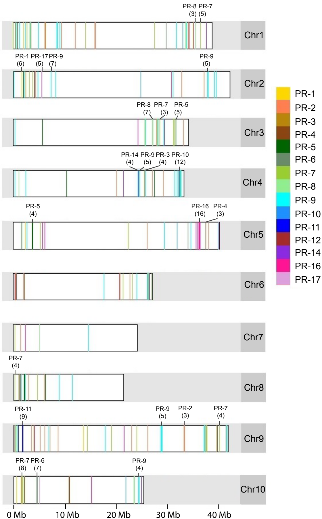
Figure S1. Karyogram depicting the position of PR genes along the length of chromosomes based on the Matina genome sequence. Tandem arrays are labelled above the chromosomes with gene family and number of genes in the array in parentheses. Length of chromosomes is shown in Mb. Due to resolution of the image, lines for physically clustered genes may overlap.
