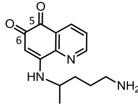
5,6-ortho-quinone
