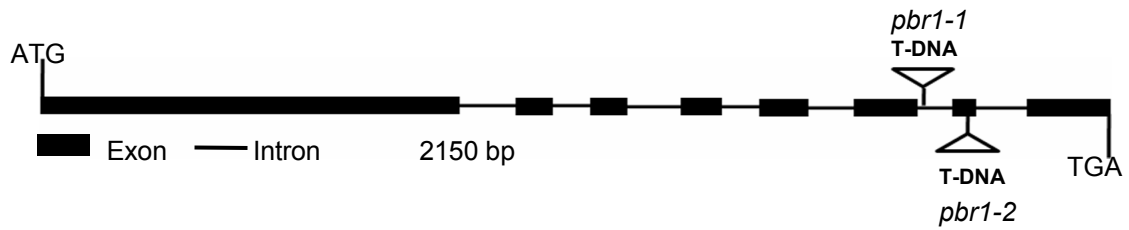
Figure S1 Schematic diagram of PBR1 gene showing the T-DNA insertion sites. Closed box indicates ORF. Exons (boxes) and introns (lines) were determined by a comparison of the genomic and cDNA sequences. The T-DNA insertion sites and positions of the start and stop codons are indicated.
