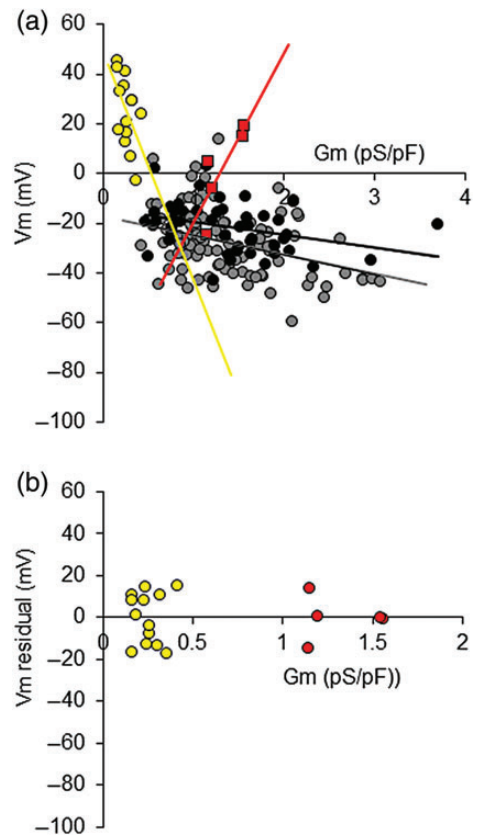
Supplementary Figure S2 (a) Scatter plot of membrane conductance ( G_m ) versus resting membrane potential ( V_m ) for individual cells from capacitated donors (black symbols), Patient C (red symbols), Patient D (yellow symbols) and all other IVF patients (grey symbols). Regression lines are presented in matching colours ( P < 0.1 , Patient C). (b) Residual plots for regressions fitted to data from patients C (red) and D (yellow). Points are randomly scattered consistent with a linear fit.
