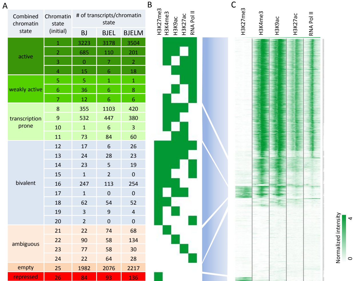
Figure S7. Chromatin state annotation. a , Statistical analysis of chromatin states (initial and combined) at the TSSs of DEGs. b , Chromatin state classification. Green box stands for the presence of epigenetic mark or polII at the TSSs \pm 500bp, white – for the absence. c , Normalized ChIP signal intensities at the TSSs \pm 500bp, ordered from 1 st to 26 th chromatin state as in (A) in BJ cells.
