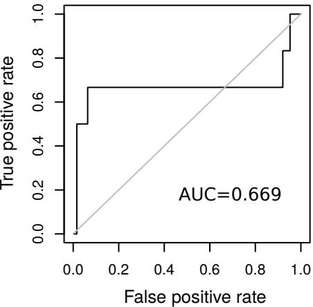
Enrichment Test
