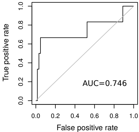
Random Forests
