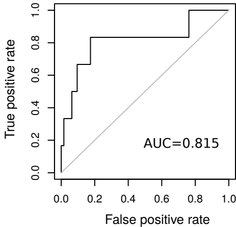
Multiple Logistic Regression
