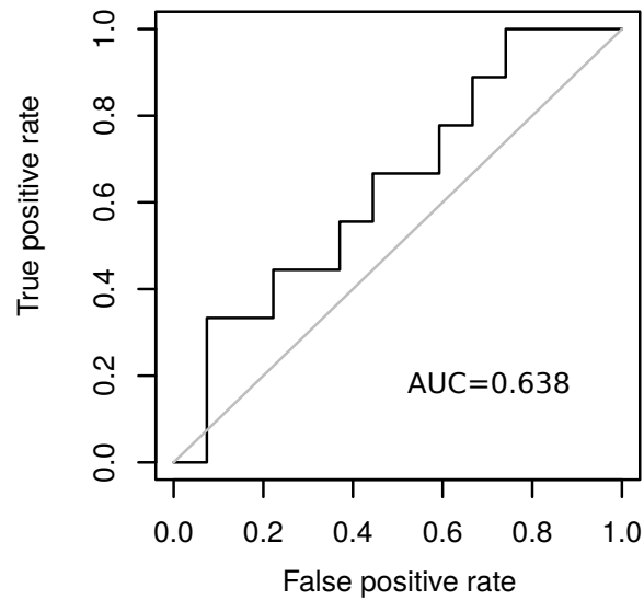
Random forests
