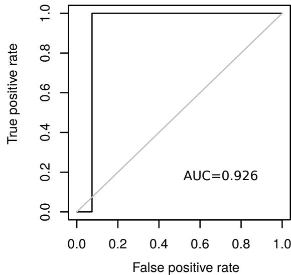
Multiple logistic regression
