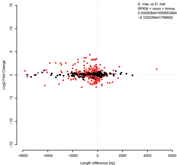
Direct Annotation
