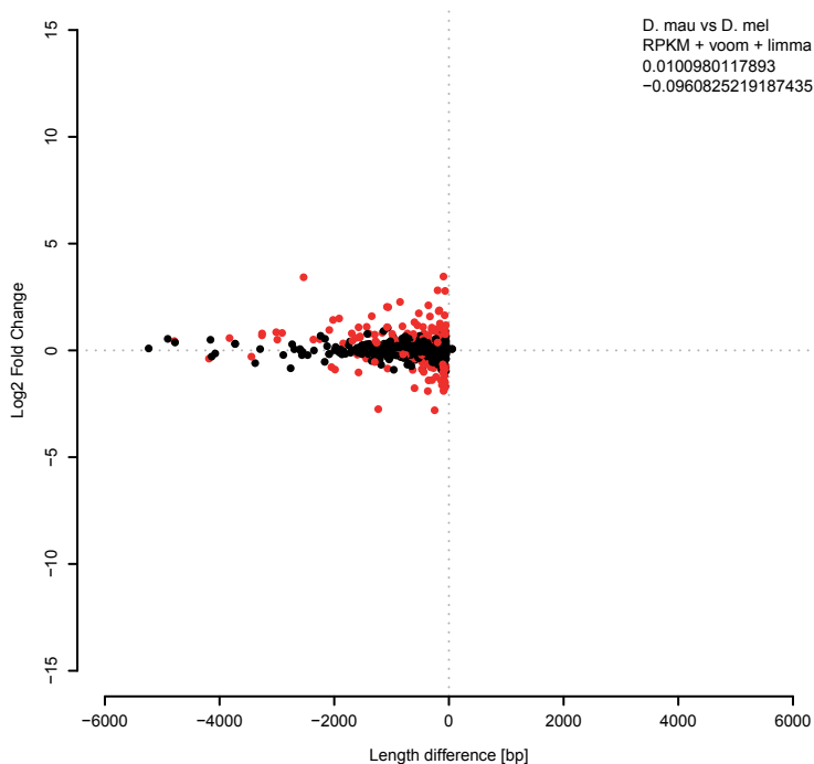
Reciprocal Annotation
