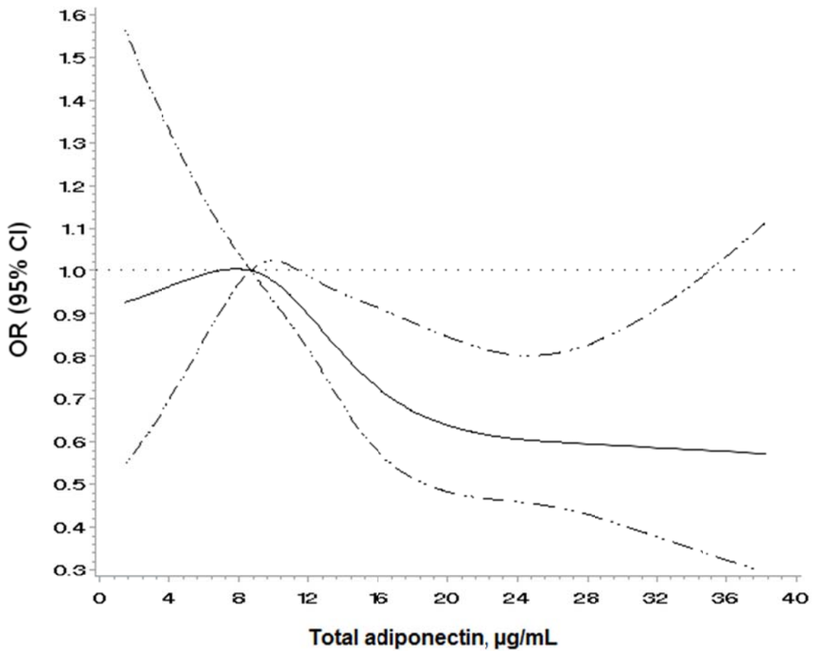
Figure S1. Risk of MM in relation to circulating total adiponectin levels estimated using a restricted cubic spline regression model with 4 knots. The odds ratio (OR) is represented by the solid line, and the upper and lower confidence intervals (CI) are represented by the dashed lines. A test for a linear relation was statistically significant ( P = 0.0007 ), and there was no evidence of departure from linearity ( P for non-linearity = 0.4).
