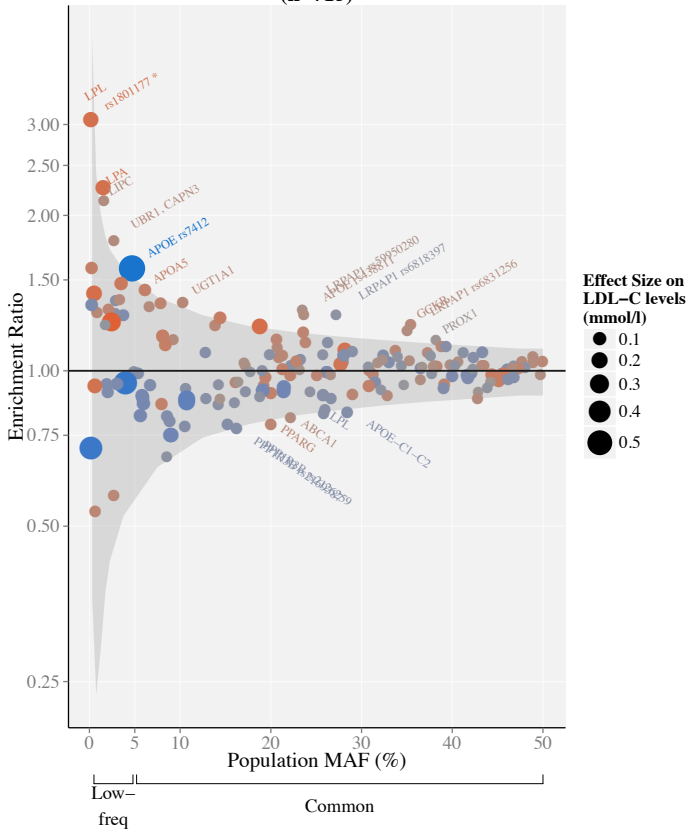
(c) All score variants in all FCH family members (n=715)
