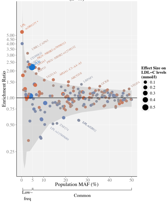
(a) All score variants in family probands (n=48)
