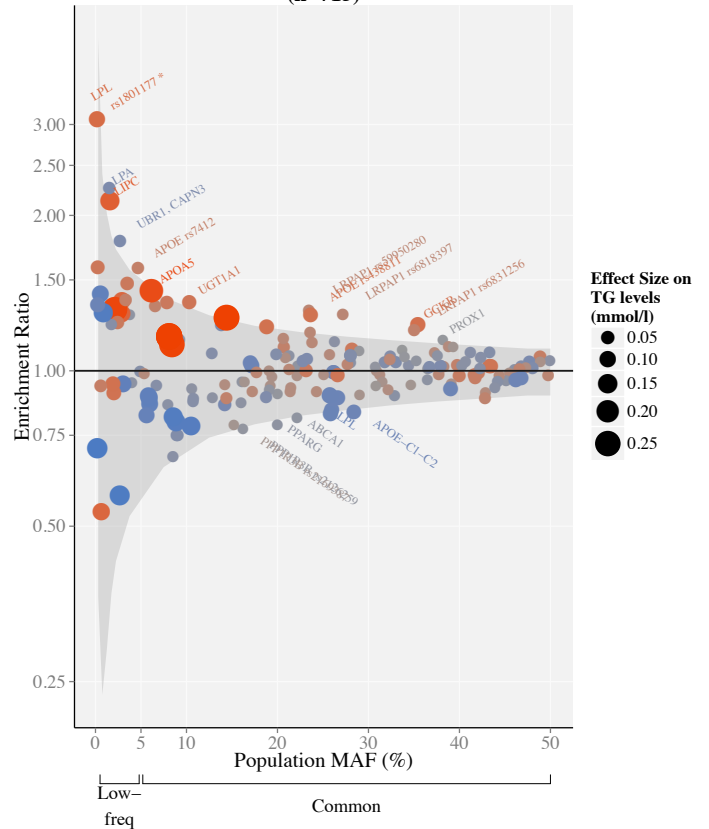
(d) All score variants in all FCH family members (n=715)
