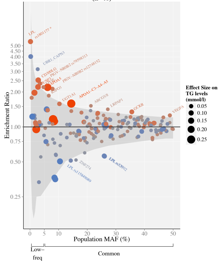
(b) All score variants in family probands (n=48)
