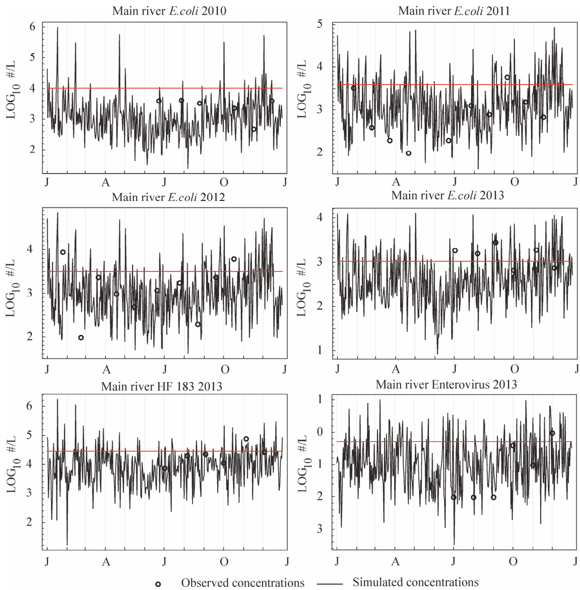
SI Figure 2: Simulated and observed concentrations of E.coli from 2010 to 2013 and of HF183_II and enterovirus in 2013 at PI
