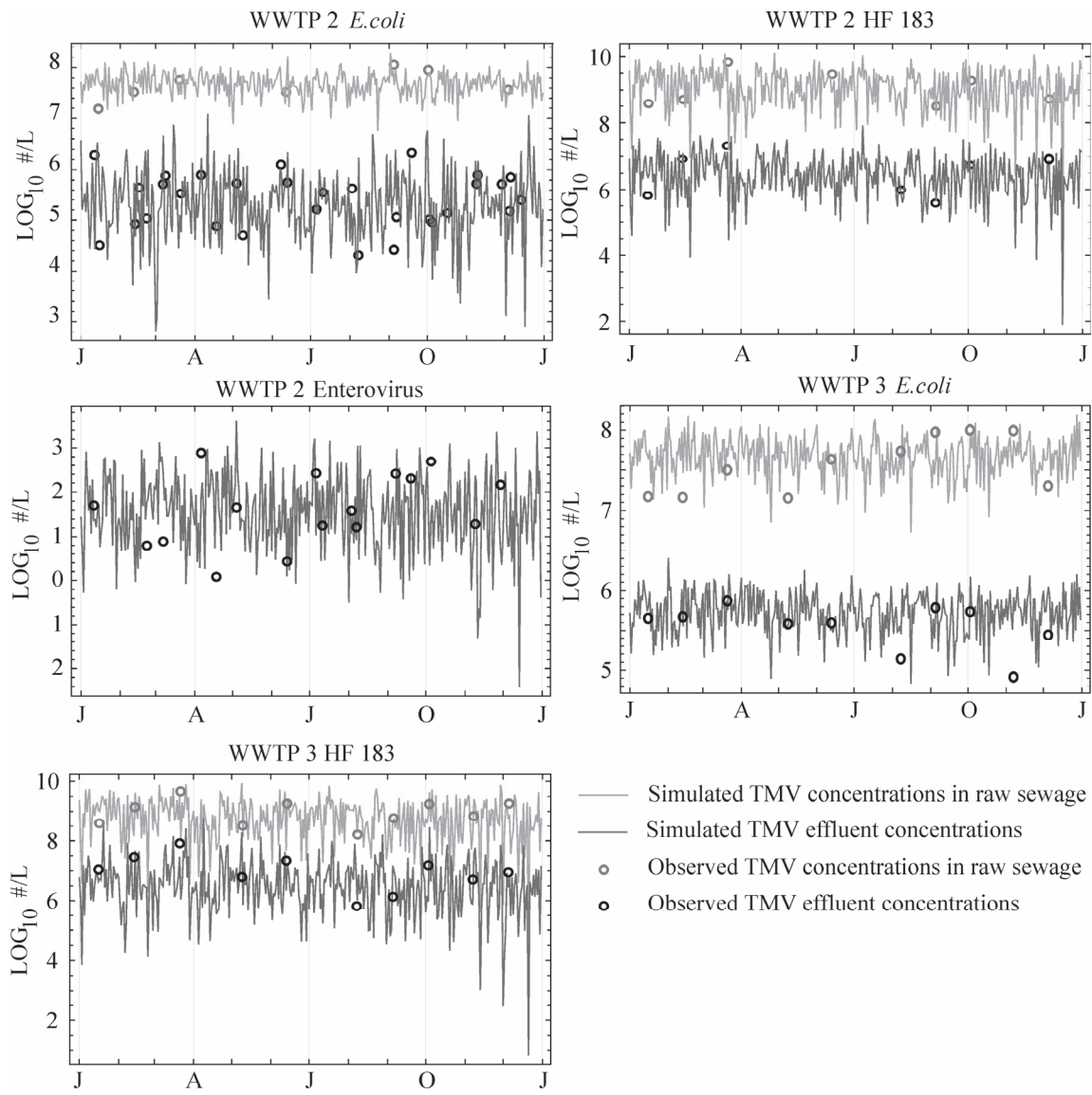
SI Figure 1: Simulated and observed concentrations in raw sewage and wastewater effluent of WWTPs 2 and 3 for enterovirus, E.coli and HF183_II based on pooled data from 2010 to 2013.
