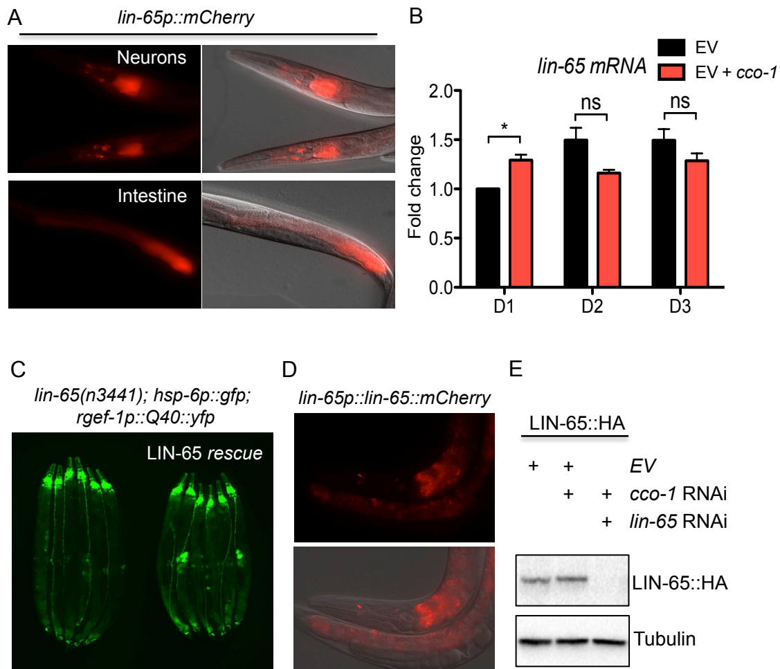
Figure S2. lin-65 is mainly expressed in the intestine and neurons, Related to Figure 2
