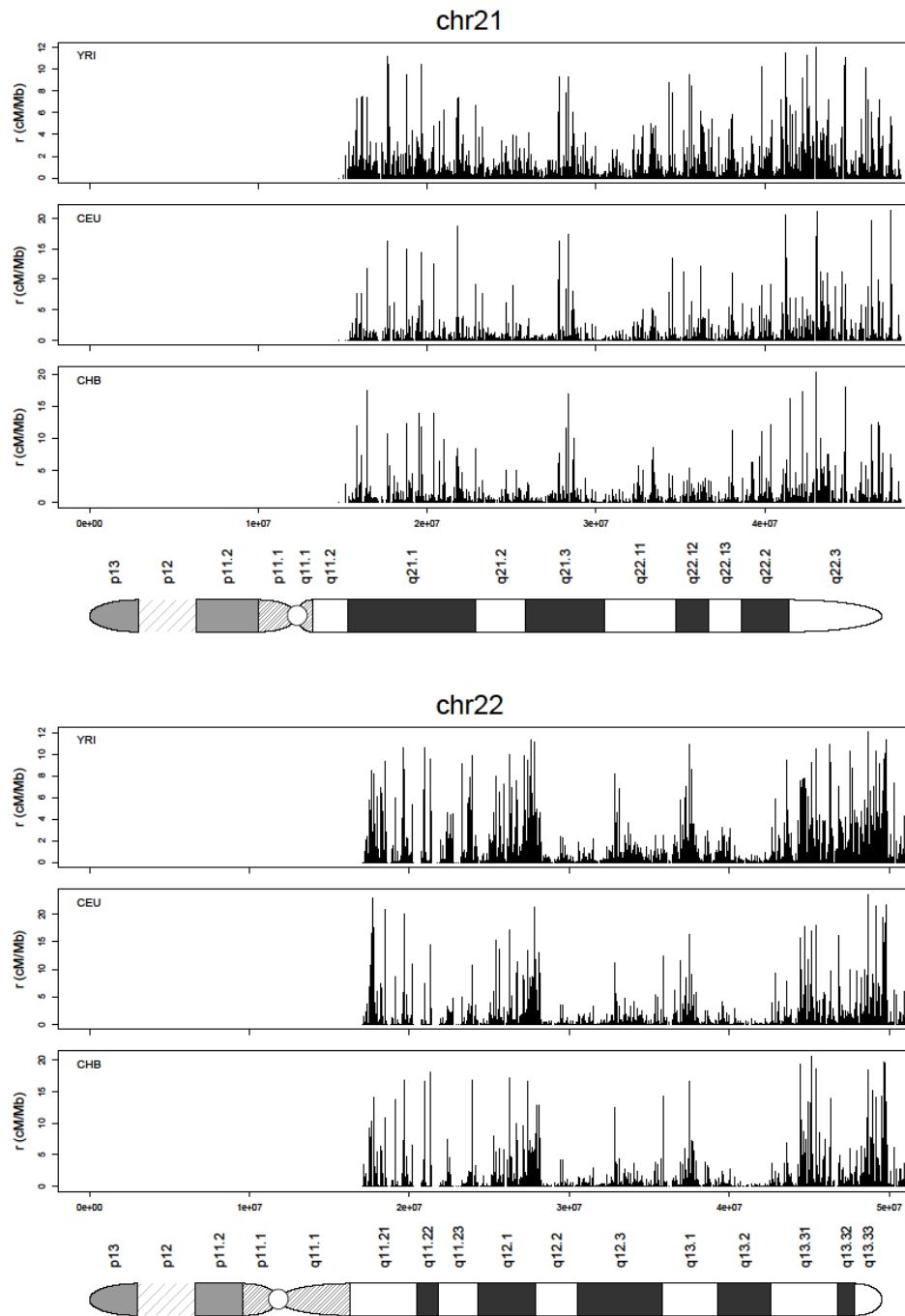
Figure S5 Recombination rates of the 22 autosomes for three human populations of African (YRI), European (CEU) and East Asian (CHB) ancestry at a 50-kb scale. The cartoon at the bottom is a visualization of the chromosome.
