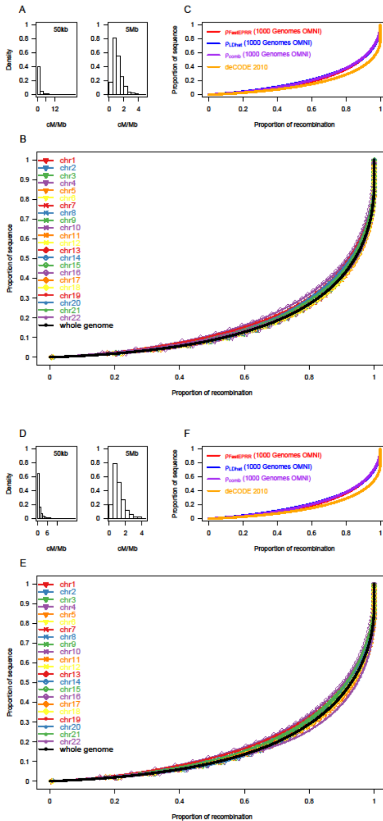
Figure S6 Recombination rate in European (CEU) (A, B, C) and East Asian (CHB) (D, E, F).
