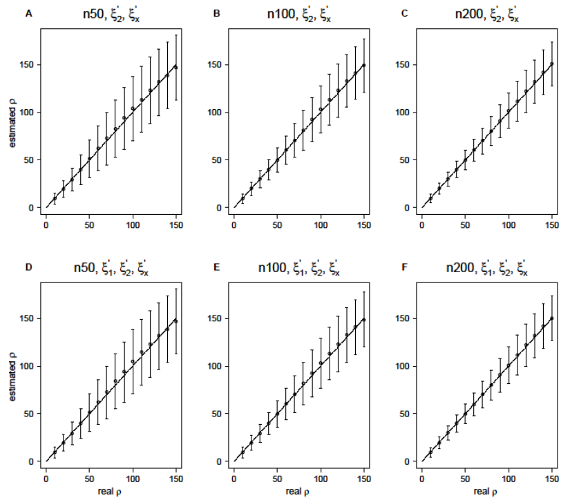
Figure S9 Comparisons of \rho_{FastEPRR} with and without \xi_1' . \hat{\rho} was estimated without \xi_1' (A-C)
