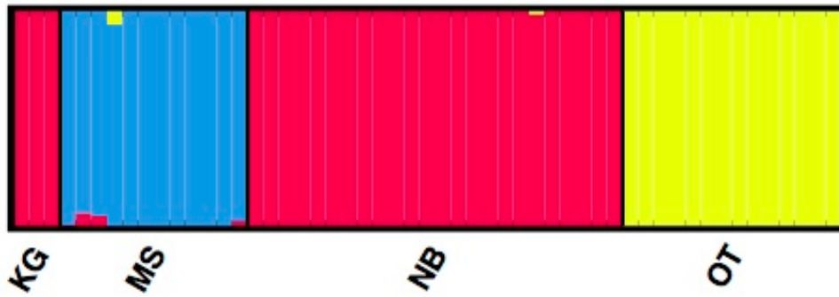
Figure S2: Genetic membership bar plot based on 73, 297 SNPs obtained using fastStructure (Raj et al. 2014). Each vertical bar represents a single individual. The height of each color represents the probability of assignment to each of K=3 clusters for all sampled flies in all populations ( N=53 ). KG: Kalangala; MS: Masindi; OT: Otuboi; NB: Namutumba.
