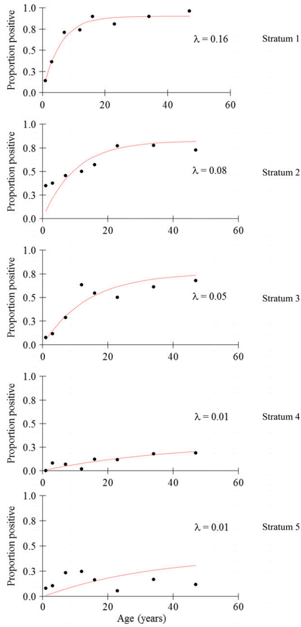
SUPPLEMENTAL FIGURE 1. Seroprevalance curves for Plasmodium falciparum merozoite surface protein-1 19 (MSP-1 19 ) antigens for each stratum, Uganda.
